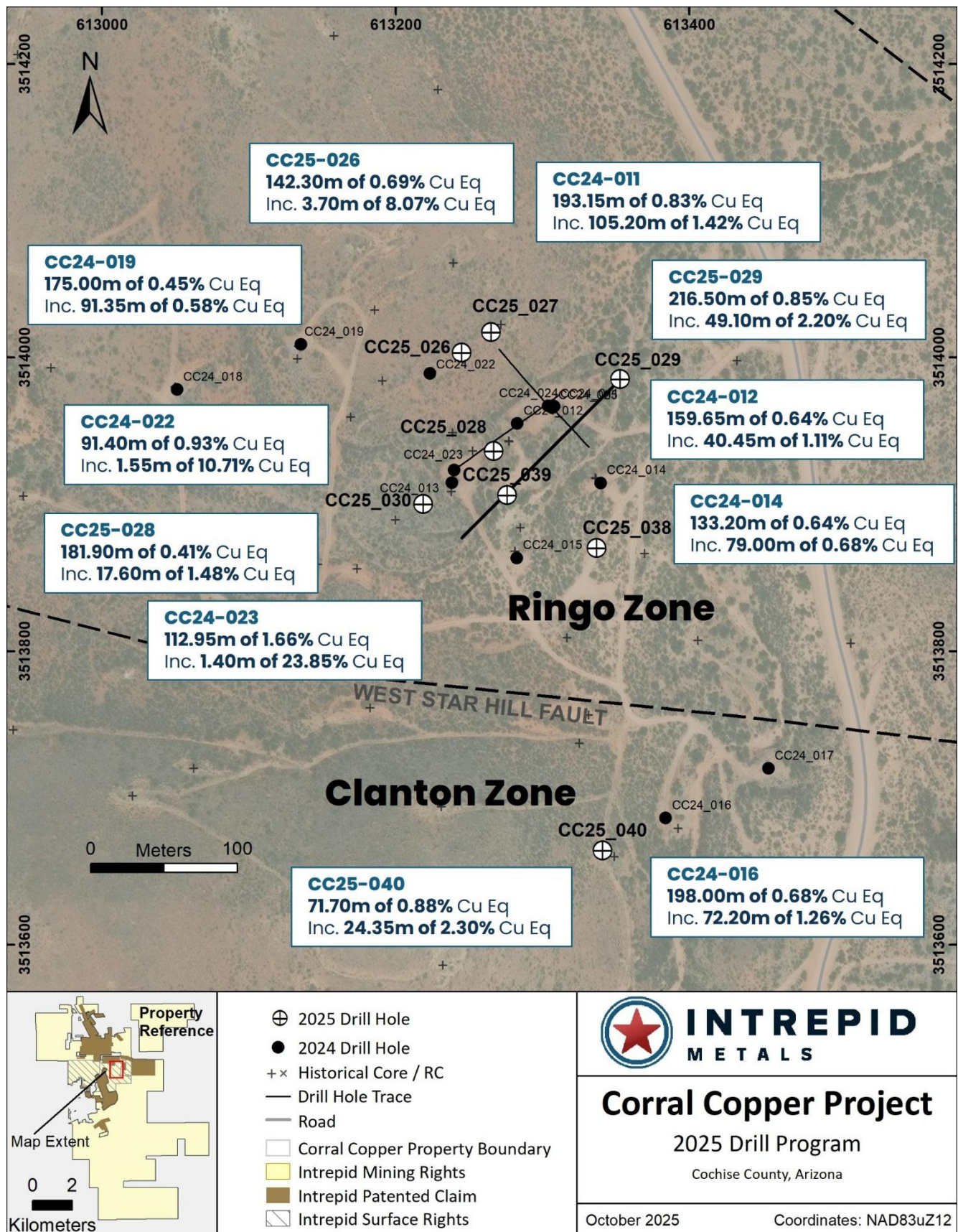
Figure 1: Drill plan map from the Ringo and Clanton Zones at Corral Copper
